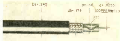
Fig. 3. Dimensions and characteristics of coaxial air-spaced low-capacitance cable
