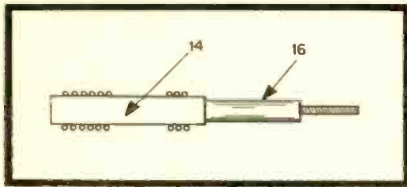
Fig. 7. Design of a single-core commercial inductor; length-to-diameter ratio is 8-to-1 or 10-to-1
