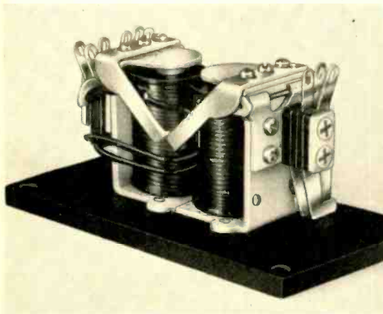
LATCHING AEROTROL showing special wiring between terminals. Any two AEROTROLS of similar or different types may be combined into a LATCHING AEROTROL while retaining the advantages of the individual relays. They offer a simple, yet positive, means of providing sequence operation of controlled circuits.
