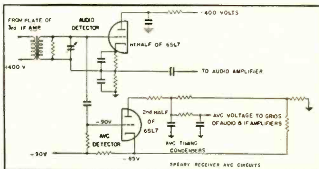
Fig. 3. Simplified schematic diagram of the audio and a-v-c detectors
