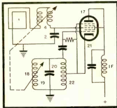
Fig. 10. Ganged inductively tuned loop and local oscillator system
