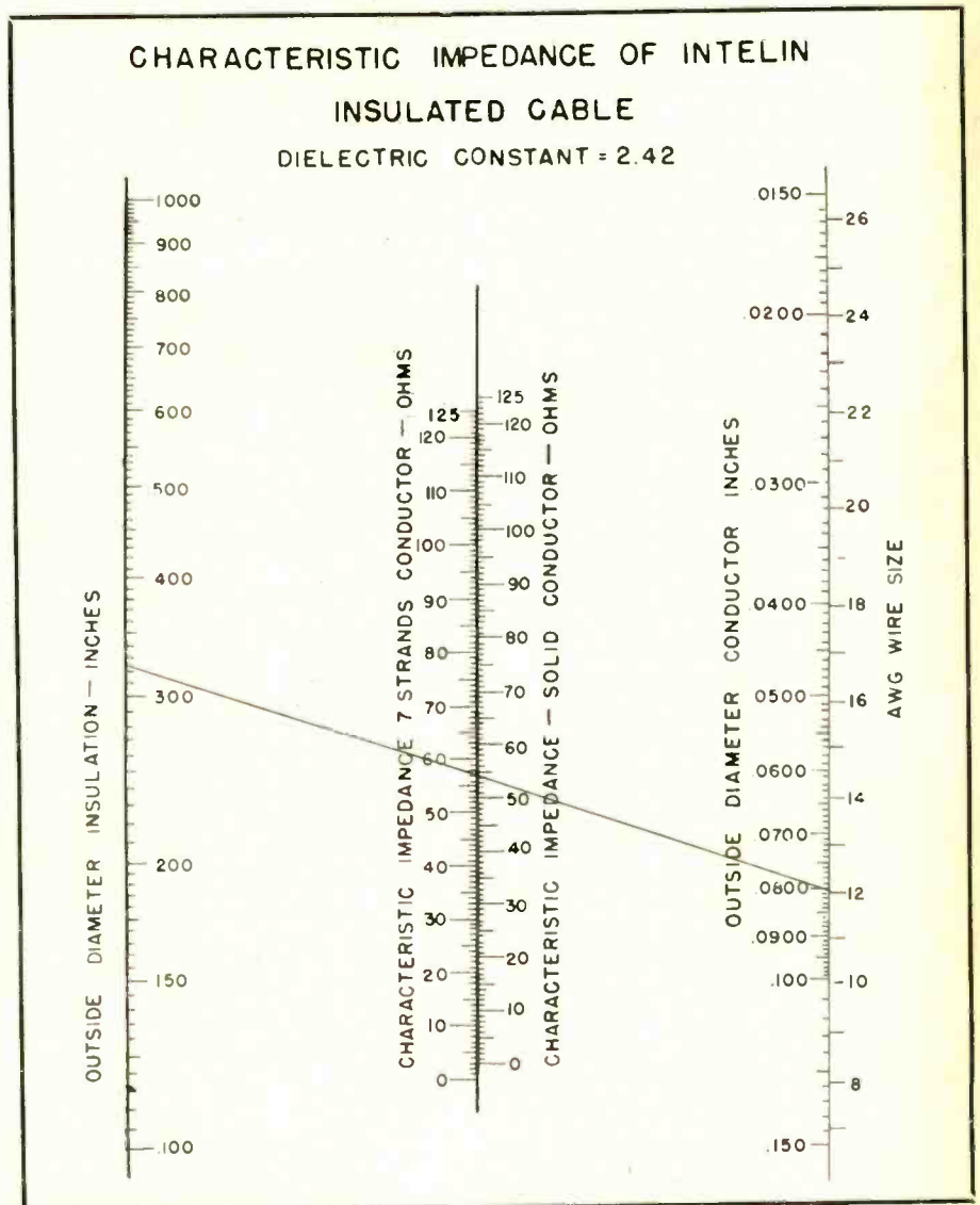
Fig. 2. Nomograph calculating the characteristic impedance of polyethylene insulated cable
