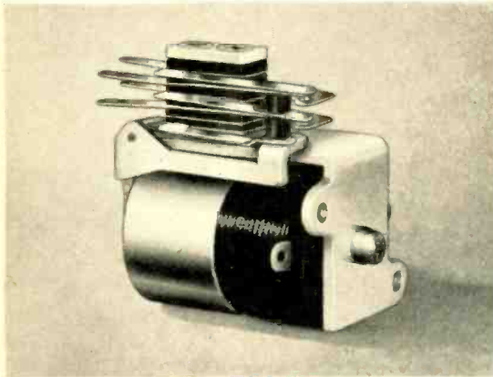
No. 400-494. Slow release AEROTROL for time-delay applications. Size 1\frac{1}{16} " x 2\frac{1}{32} " x 1\frac{3}{8} ". Weight 3.5 ounces. Operating voltage 24 volts D.C. Operating time 8 milliseconds. Release time 35 milliseconds. Minimum operation .085 amperes.
