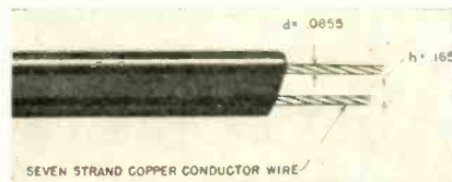
Fig. 7. A typical example of the less expensive antenna lead-in wire which will find wide application in the FM and television receiver field
