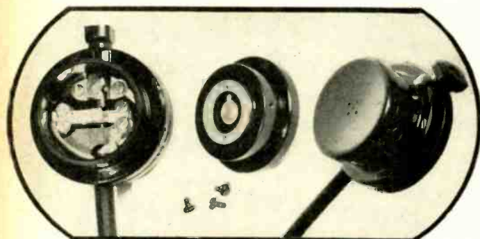
Anti-noise carbon microphone as used in modern police equipment. It features low-frequency response and rugged recessed mouthpiece for good signal-to-noise ratio — Aviometer photo.
