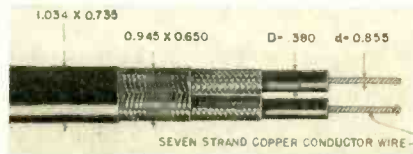
Fig. 5. Dual Coaxial cable used when a high degree of balance precision is necessary
