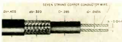
Fig. 6. Dimensions and characteristics of a dual twinax cable which also achieves a high degree of balance
