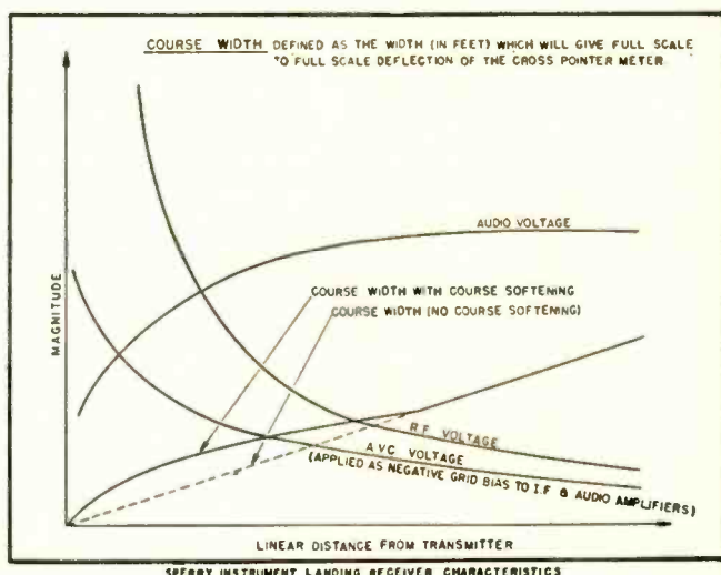
Fig. 4. A-v-c action produces relative course-softening, as graphed.
