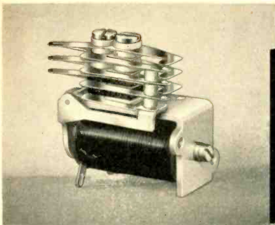
No. 400-452. Single pile up AEROTROL with combination Bakelite-Cecotite insulation for maximum insulation and low capacitance. Size 1\frac{1}{16} " x 2\frac{1}{32} " x 1\frac{1}{32} "; Weight 2 ounces. Operating voltage 14 volts D.C. Minimum operation .045 amperes. Coil resistance 280 ohms.
